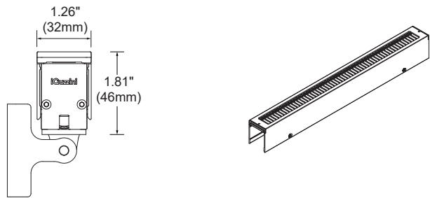
A5- Honeycomb louver
