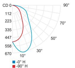
Wall washer (3000K, 92CRI)
