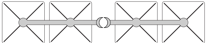
B2 - DOUBLE HORIZONTAL TWO Arm length: Small: 2 x 30 1 / 8 " (840mm) Large: 2 x 47 1 / 8 " (1196mm)
