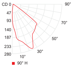
BO blade effect (3000K, 80CRI)
