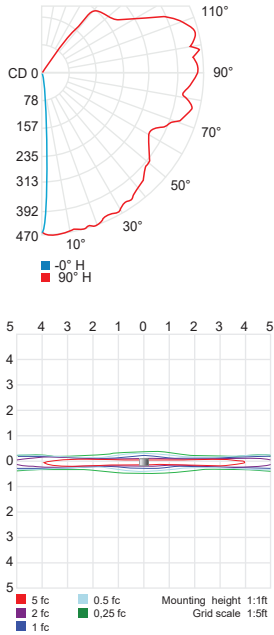
BO 360° blade effect (3000K, 80CRI)
